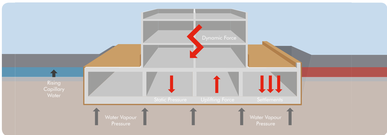
FIGURE 1: Forces Impacting on the Multi Storey Car Park
